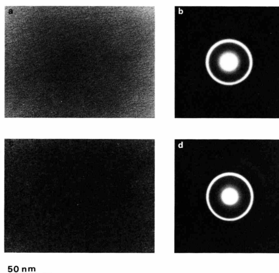
Fig. 1. Bright field electron micrographs (a, c), and selected area diffraction patterns (b, d) of an amorphous \text{Al}_{75}\text{Cu}_{15}\text{V}_{10} alloy aged for 40 800 sec (a, b) and 86 400 sec (c, d) at 620 K.
